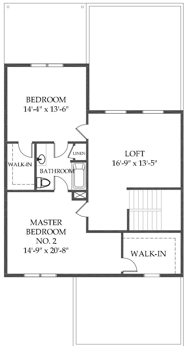
2ND FLOOR
