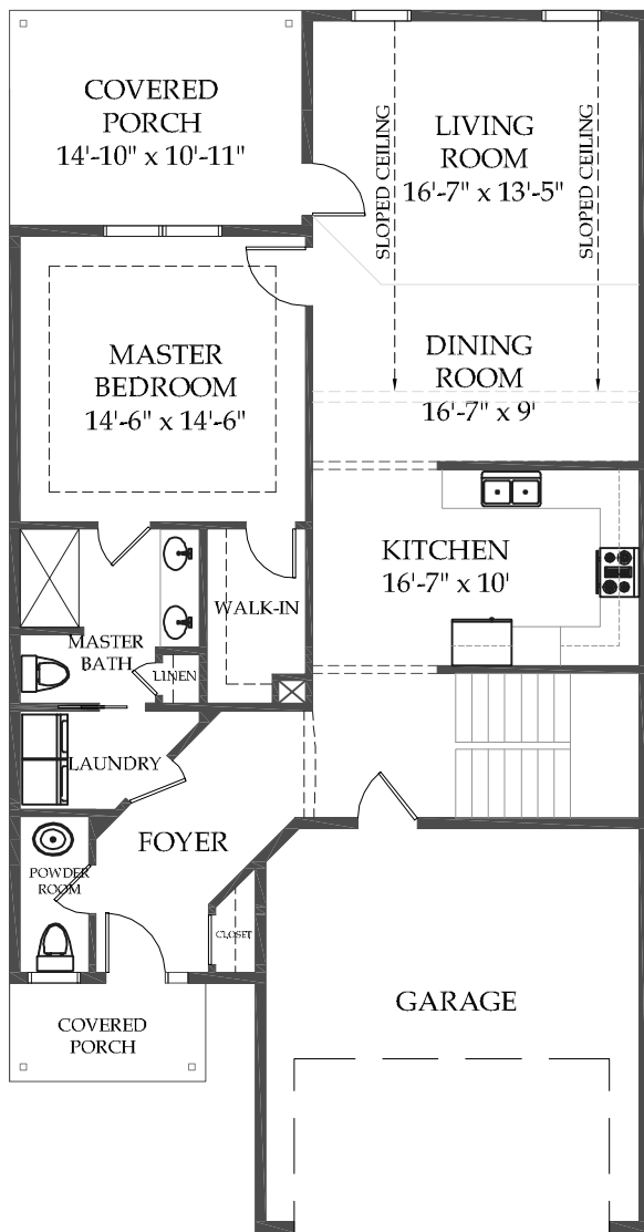
1ST FLOOR
